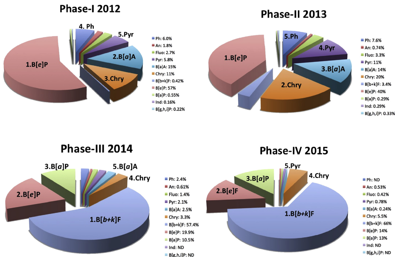
Fig. 2. Percentage contribution of PM 2.5 -bound PAHs collected at nine administrative provinces of Northern Thailand during four different periods.
