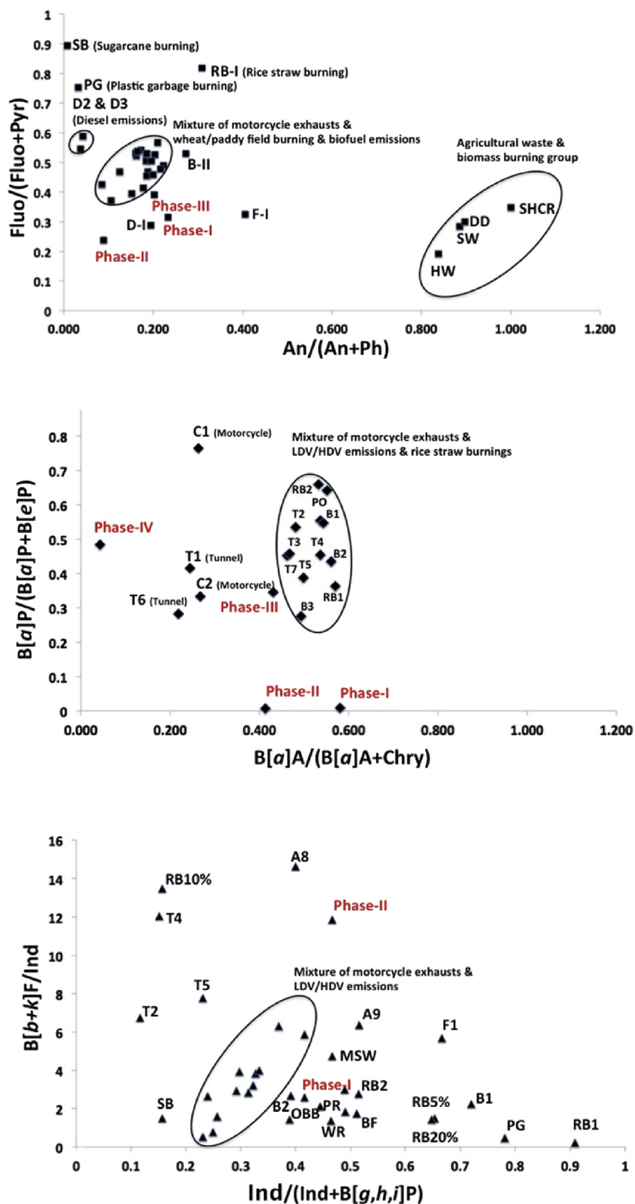
Fig. 4. Diagnostic binary ratios of PM 2.5 -bound PAHs in the NNP.
