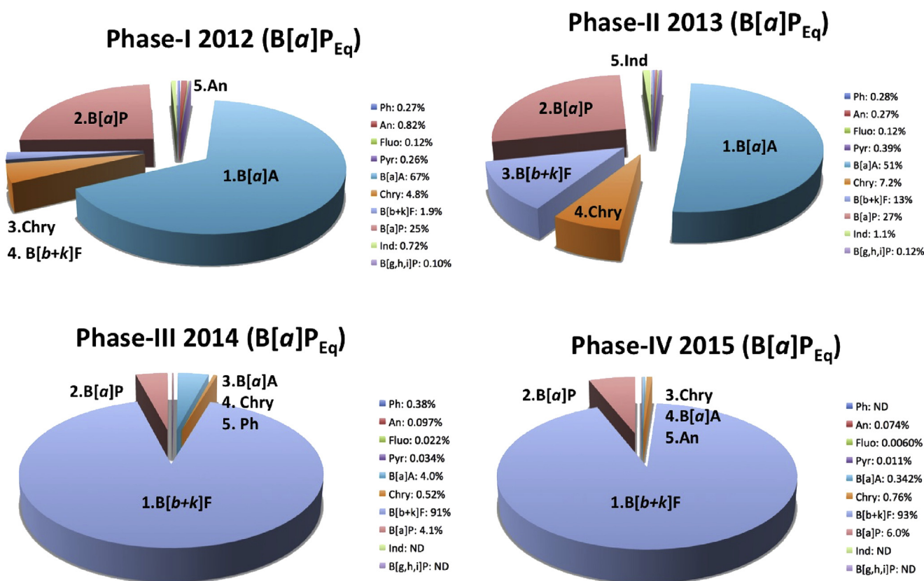
Fig. 3. Percentage contribution of B[a]P_{Eq} of PM_{2.5} -bound PAHs collected at nine administrative provinces of Northern Thailand during four different periods calculated using Nisbet and Lagoy's equation.
