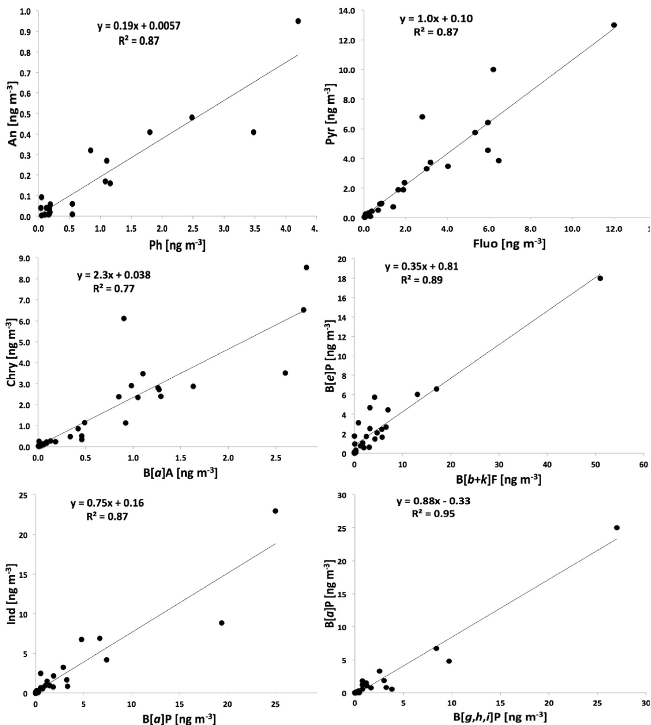
Fig. 5. Linear regression analysis of PM 2.5 -bound PAHs in the NNP (Phases I-IV), in comparison with other urban areas (Afghanistan (Wingfors et al., 2011), Belgium (Ravindra et al., 2006), Brazil (Bourotte et al., 2005; Silva et al., 2010), China (Deng et al., 2006; Gao et al., 2011; Hou et al., 2006; Li et al., 2005; Wang et al., 2006), Germany (Schnelle-Kreis et al., 2005), Hong Kong (Guo et al., 2003), Italy (Vassura et al., 2014), Japan (Naser et al., 2008), Singapore (Karthikeyan et al., 2006), Spain (Barrado et al., 2012; Reche et al., 2012), Sweden (Wingfors et al., 2001, 2011), Taiwan (Fang et al., 2005), USA (Chellam et al., 2005; Poor et al., 2004)).
