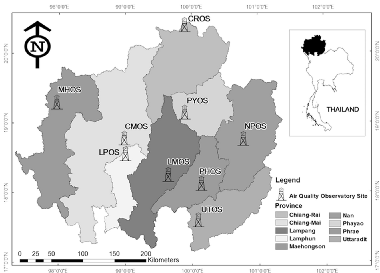
Fig. 1. Map showing location of air quality observatory sites in the nine administrative provinces of Northern Thailand (Table S.1). Please see the following references for more details of air quality observatory sites (Pongpiachan, 2016; Pongpiachan et al., 2015a).
