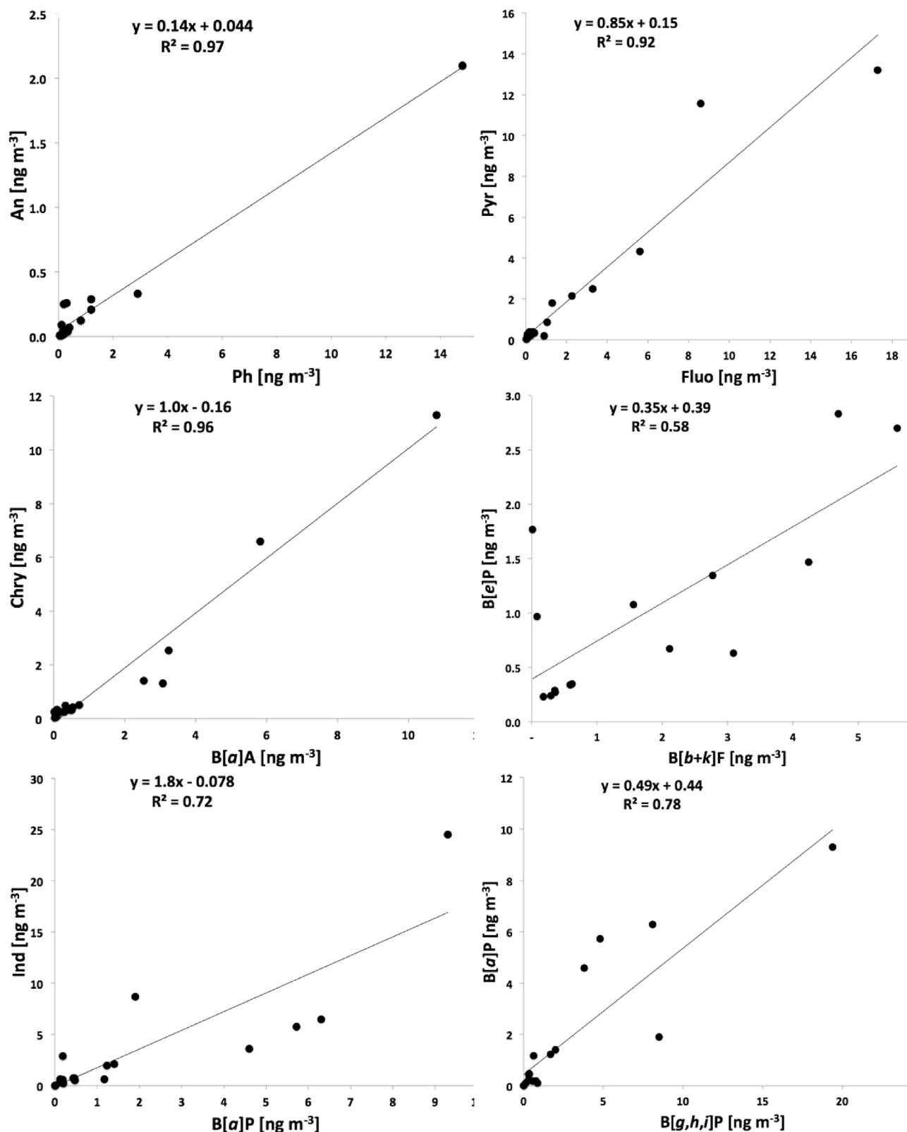
Fig. 6. Linear regression analysis of PM 2.5 -bound PAHs in the NNP (Phases I-IV), in comparison with other biomass/agricultural waste burnings (agricultural waste/biomass burnings (Pongpiachan, 2014a), bonfire (Pongpiachan, 2013a; Vassura et al., 2014), domestic heating (Ma et al., 2010), and sugarcane open burning (Godoi et al., 2004; Mugica-Alvarez et al., 2015; Silva et al., 2010)).
